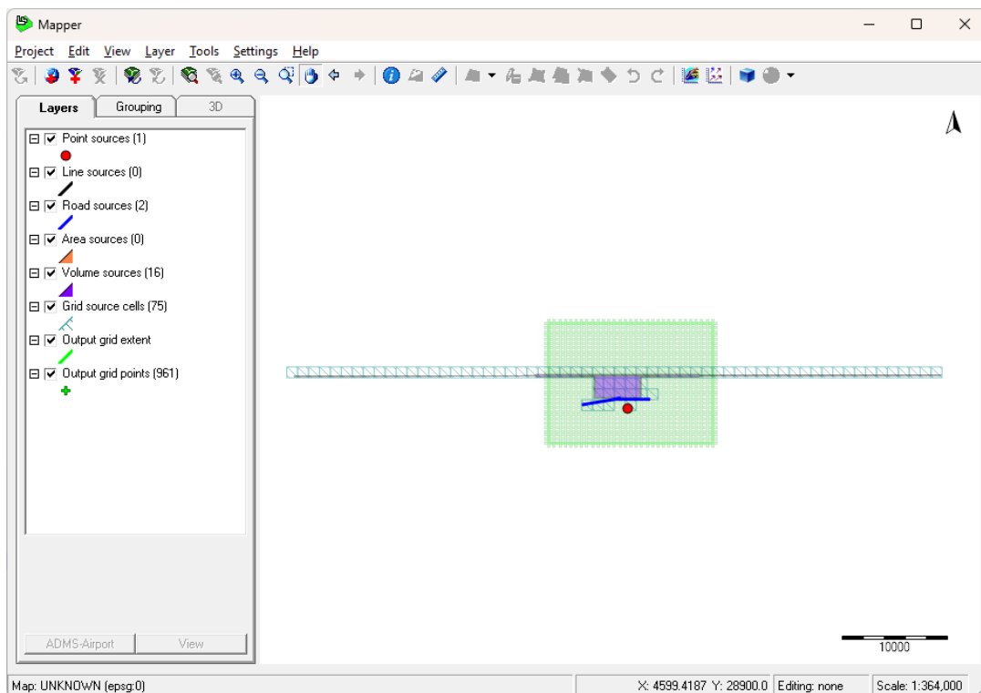
Figure 6.6 – Example 9 ADMS-Airport Sources.
