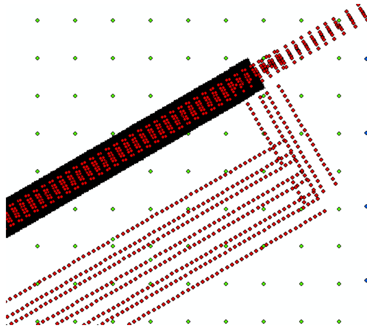
Figure 6.21 – CAEPPort case study receptor locations for generation of contour plots – close up on aircraft runway and aircraft taxiing sources ● Outer grid point, ● Inner grid point, ● Source-oriented grid point
