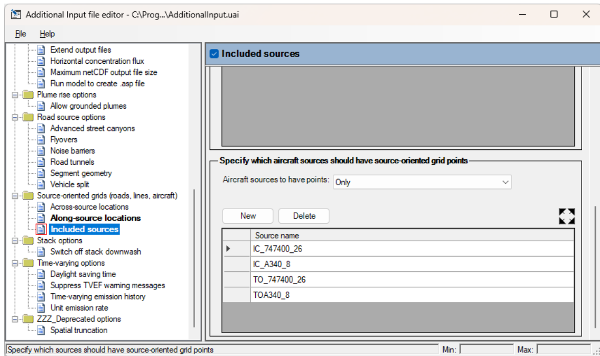
Figure 6.15 – The Included Sources section of the Additional Input File editor.
