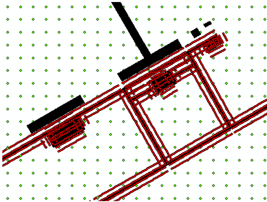
Figure 6.22 – CAEPport case study receptor locations for generation of contour plots – close up on road sources ● Outer grid point, ● Inner grid point, ● Source-oriented grid point
