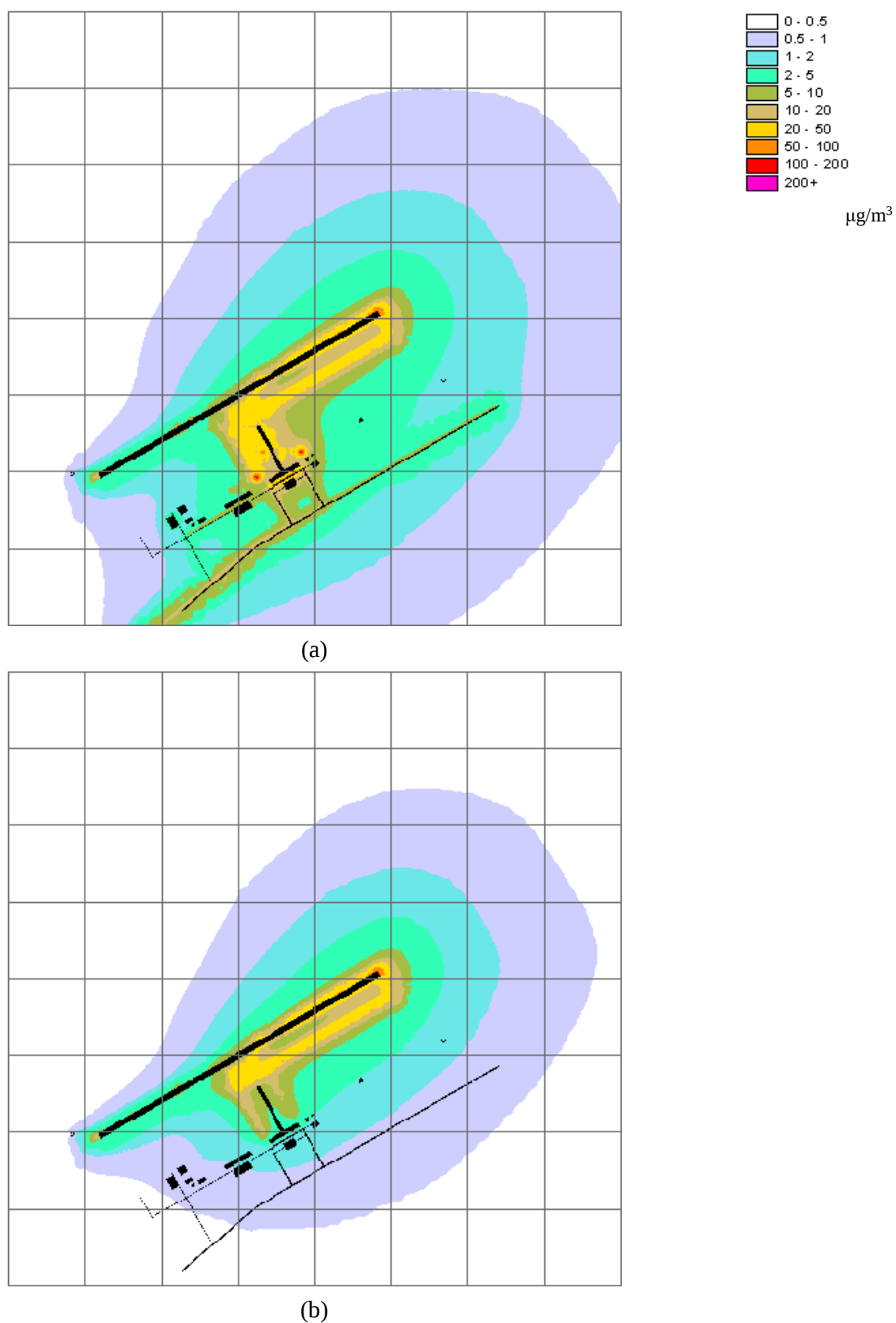
Figure 6.25 – CAEPport \text{NO}_x contours (in \mu\text{g}/\text{m}^3 ) – (a) All Sources annual hourly mean, (b) Aircraft Sources annual hourly mean.
