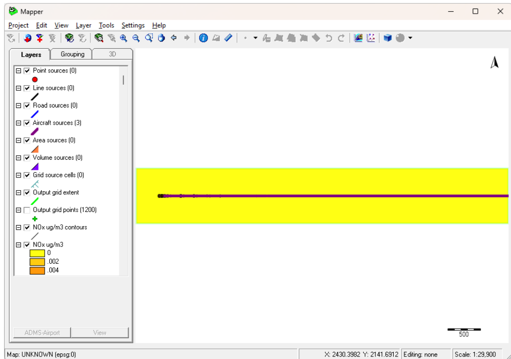
Figure 6.4 – Example 7 results of modelling an aircraft departure with aircraft sources.
