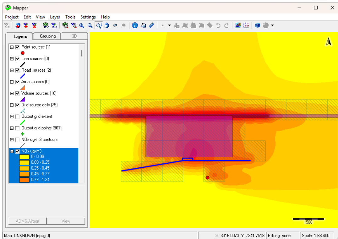
Figure 6.7 – Example 9a NO x contour plot for a simple airport
