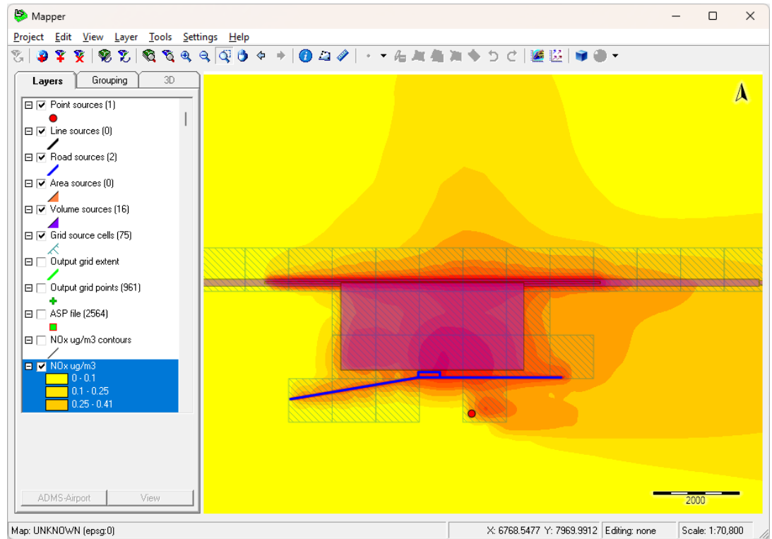
Figure 6.10 – Example 9b NO x contour plot for a simple airport
