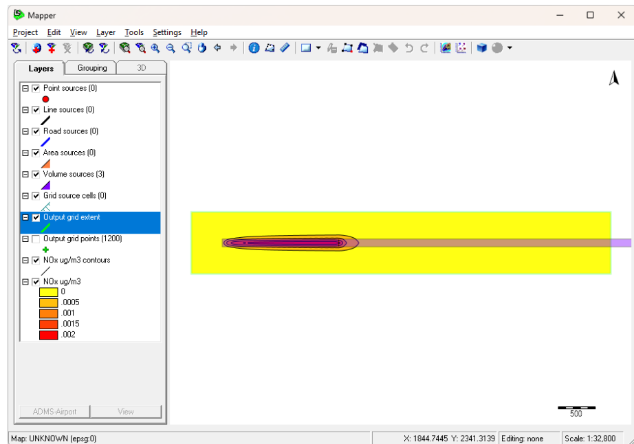
Figure 6.1 – Example 7: NO x contours for modelling an aircraft departure with volume sources.
