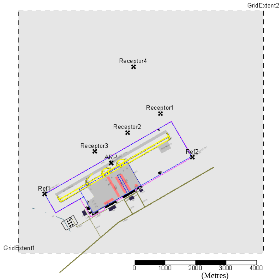
Figure 6.18 – Map of CAEPport case study receptor locations and grid extents.
