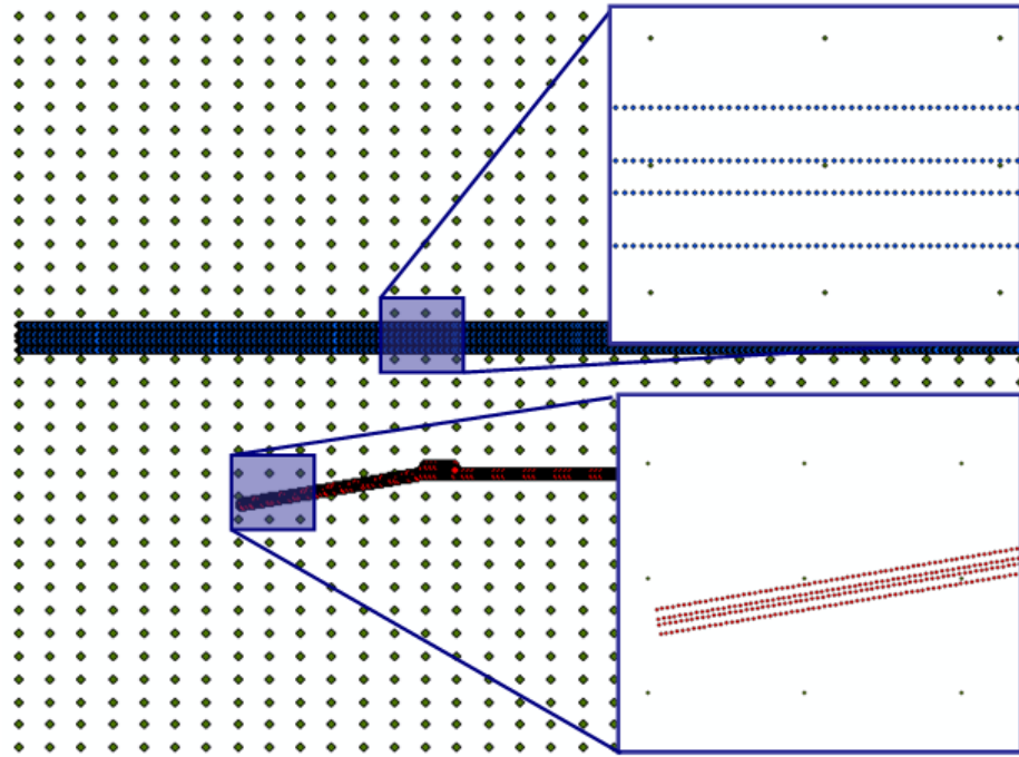
Figure 6.8 – Example 9 receptor locations for generation of contour plots ● Regular grid point, ● Source-oriented (road) grid point, ● Additional specified point
