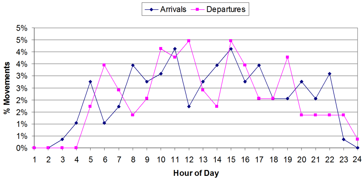
Figure 6.12 – Example 10 temporal distribution of daily aircraft arrivals and departures.
