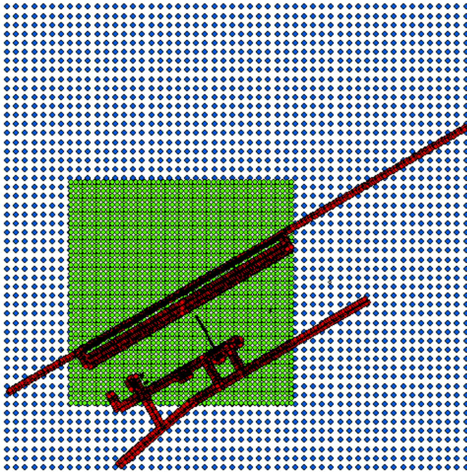
Figure 6.20 – CAEPPort case study receptor locations for generation of contour plots ● Outer grid point, ● Inner grid point, ● Source-oriented grid point
