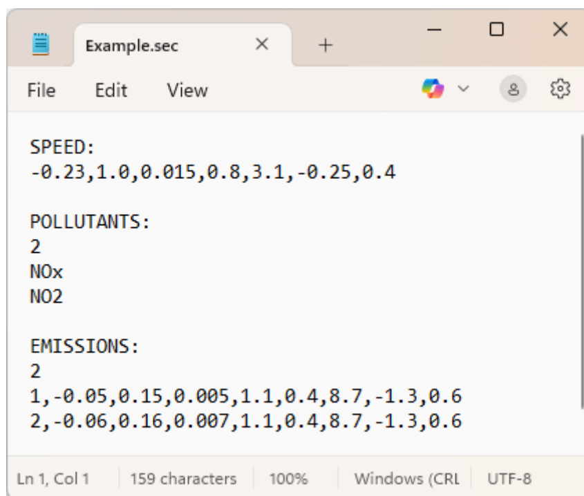
Figure 7.4 – An example of a .sec file
