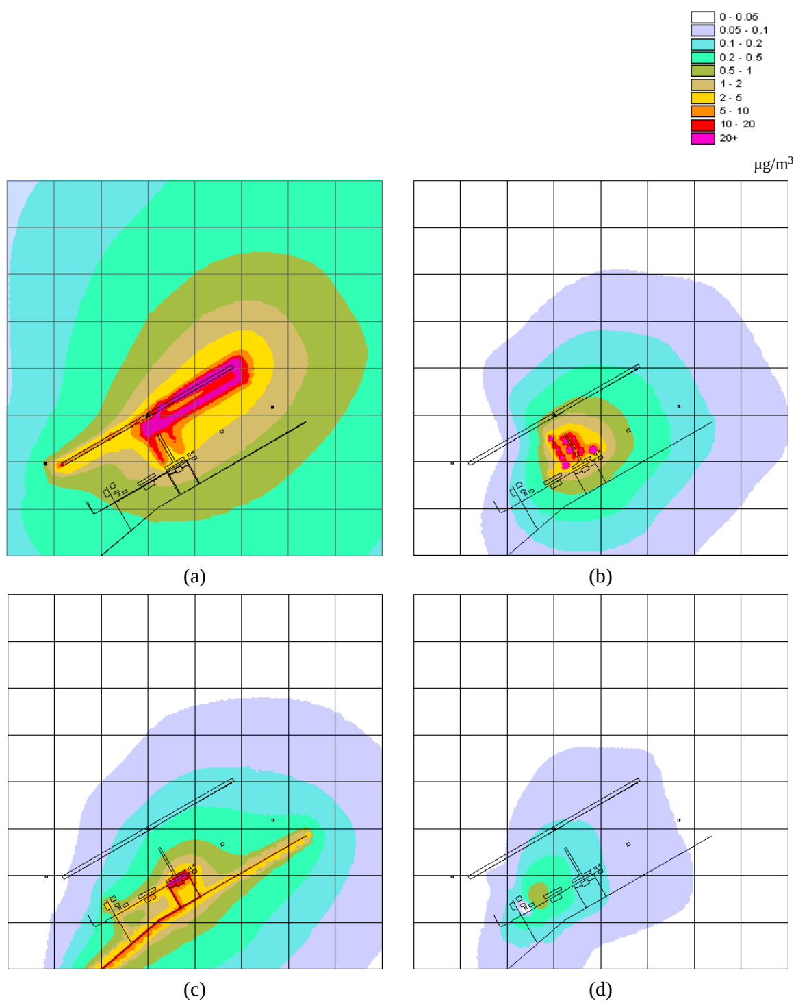
Figure 6.26 – CAEPport case study annual mean \text{NO}_x concentration contours ( \mu\text{g}/\text{m}^3 ) for (a) aircraft sources, (b) APU & GSE sources, (c) road traffic sources and (d) stationary sources.
