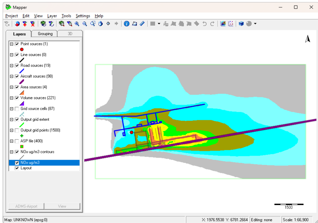
Figure 6.16 – Example 10 NO x contour plot for a complex airport
