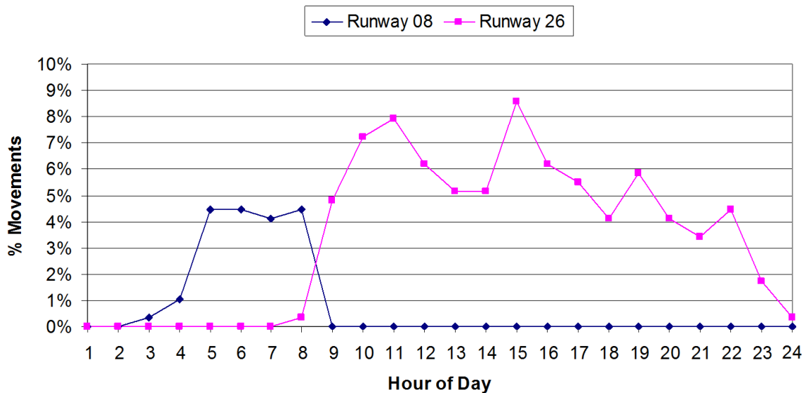
Figure 6.13 – Example 10 temporal distribution of daily aircraft movements for each runway.
