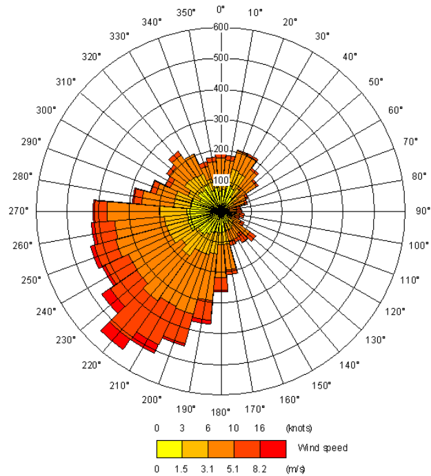
Figure 6.19 – CAEPport wind rose of meteorological data.
