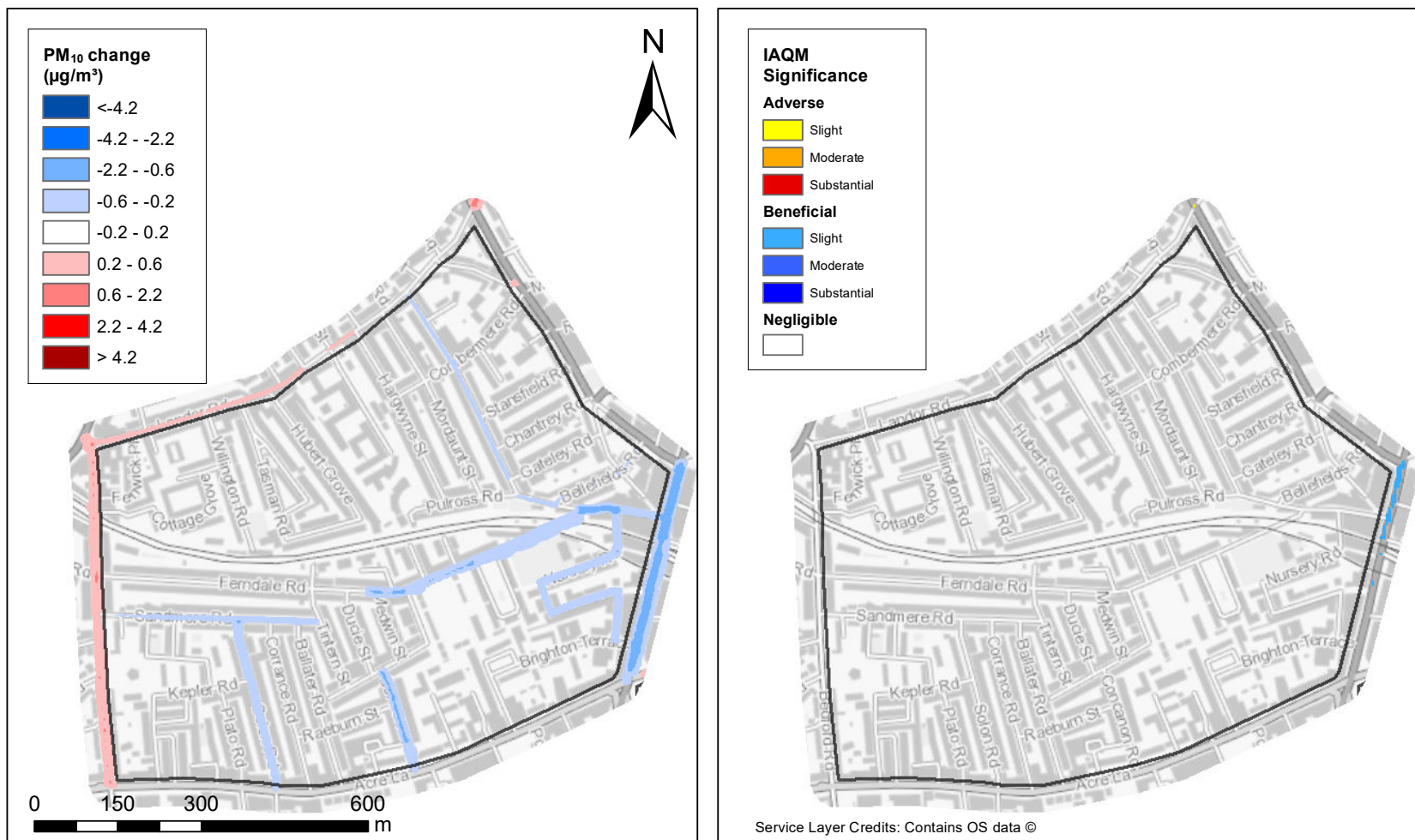
Figure 6.8: Difference plot (post-scheme minus pre-scheme) of annual average PM_{10} concentrations coloured by EPUK IAQM concentration change bands (left) and impact descriptor plot coloured by EPUK IAQM significance criteria (right), Ferndale LTN
