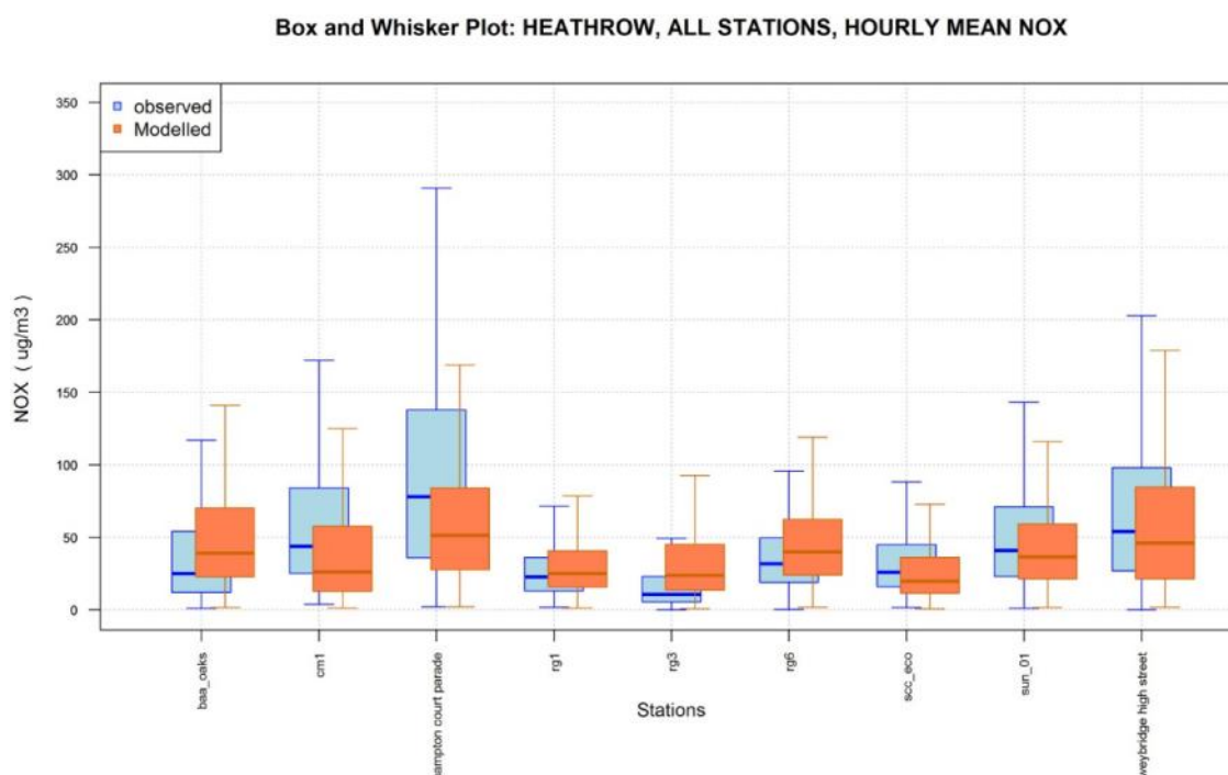
Figure 7.4: Box plots of measured and modelled hourly mean NO x concentrations at continuous monitoring sites
