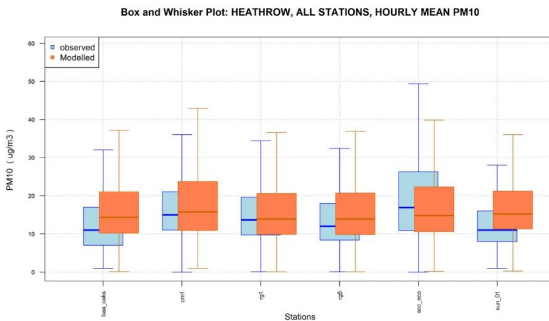
Figure 7.5: Box plots of measured and modelled hourly mean PM 10 concentrations at continuous monitoring sites
