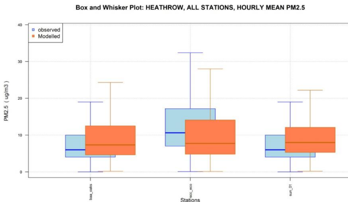
Figure 7.6: Box plots of measured and modelled hourly mean PM 2.5 concentrations at continuous monitoring sites
