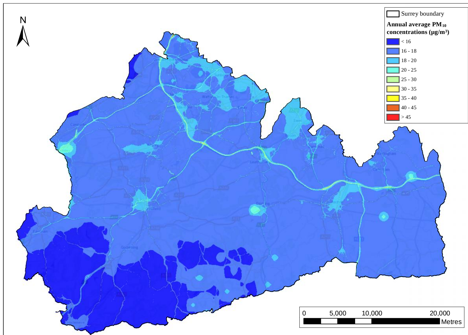
Figure 8.3: Annual mean PM_{10} concentrations, 2017 ( \mu g/m^3 )
