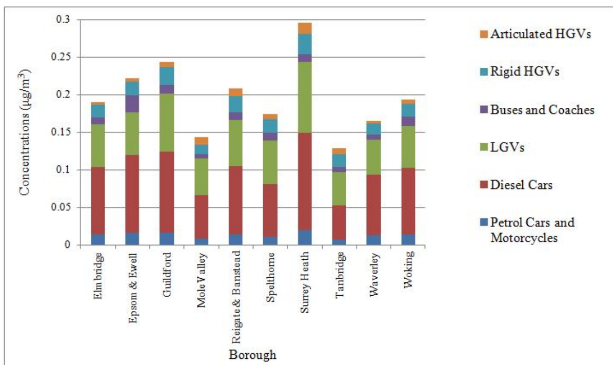
Figure 10.12: Road transport exhaust PM_{10} concentrations by vehicle category, averaged by borough
