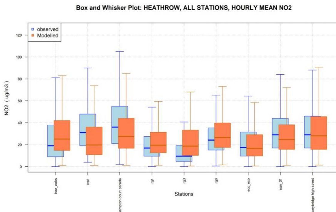
Figure 7.3: Box plots of measured and modelled hourly mean \text{NO}_2 concentrations at continuous monitoring sites
