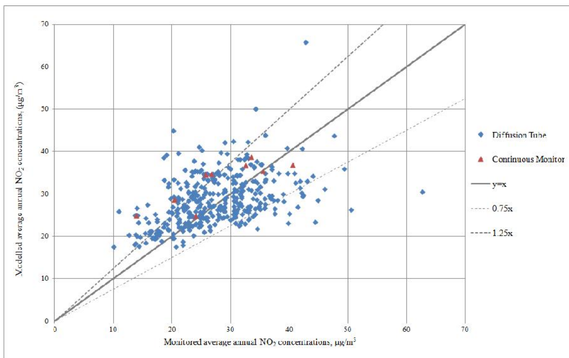
Figure B.2: Surrey measured and modelled annual average \text{NO}_2 concentrations using Gatwick meteorological data
