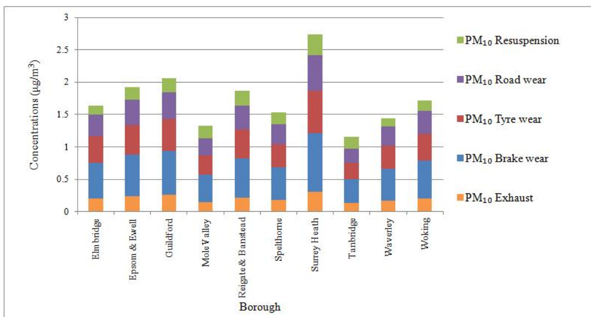
Figure 10.13: Road transport PM_{10} concentrations by exhaust and non-exhaust components, averaged by borough
