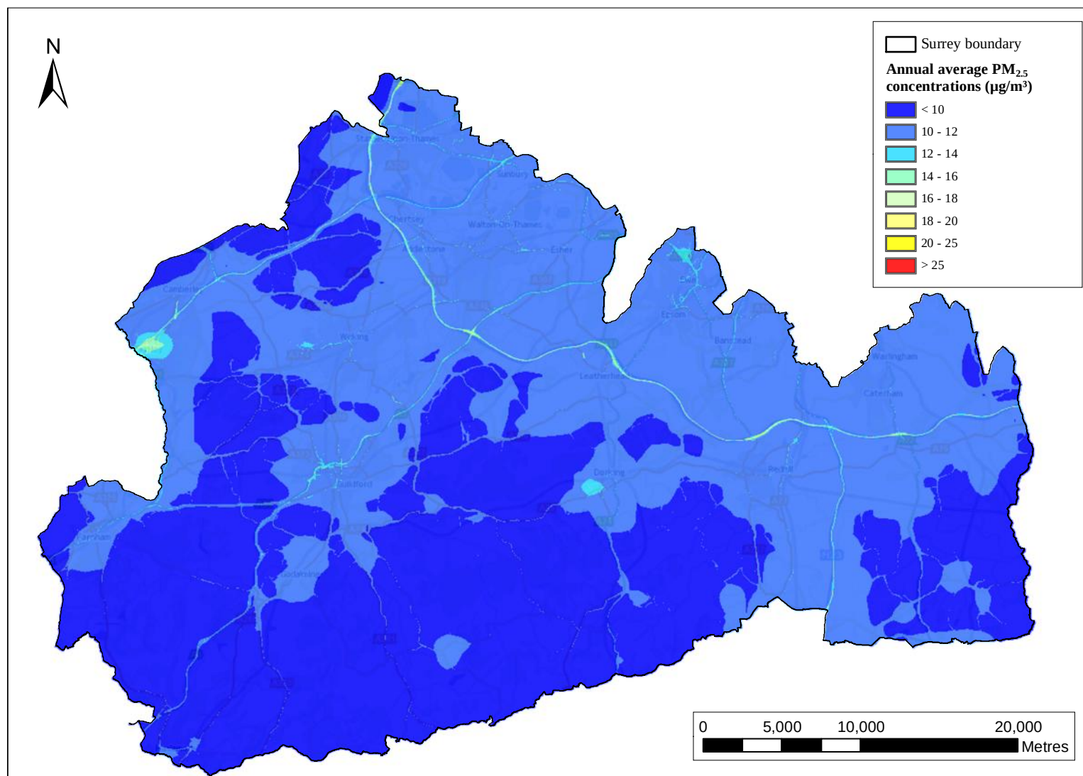
Figure 8.5: Annual mean PM_{2.5} concentrations, 2017 ( \mu g/m^3 )
