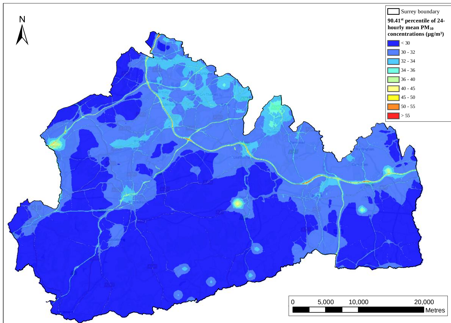
Figure 8.4: 90.41 st percentile of 24-hourly mean PM 10 concentrations, 2017 (µg/m 3 )
