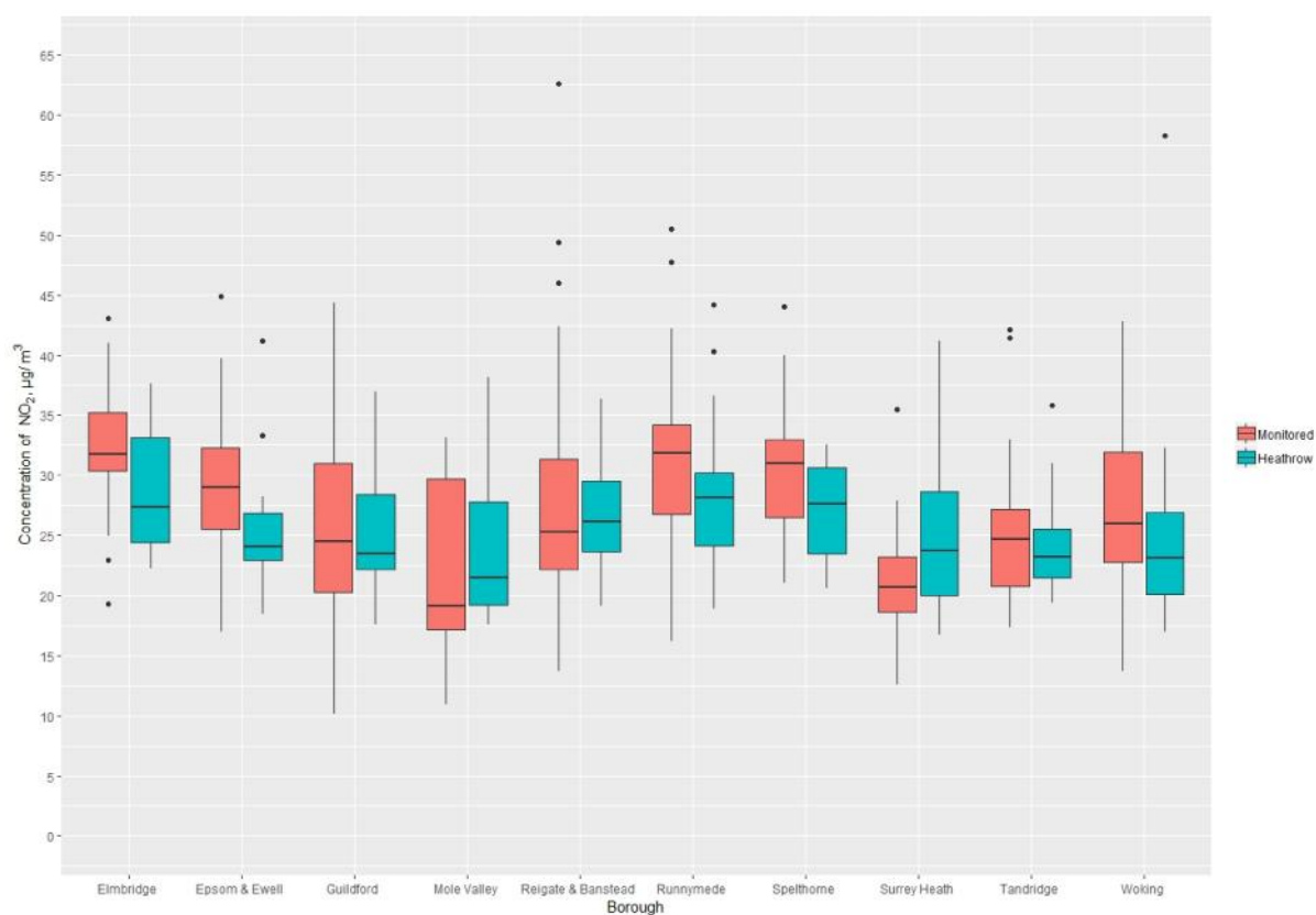
Figure 7.2: Box plots showing the spread of measured and modelled annual average \text{NO}_2 concentrations by Surrey borough. In this plot ‘outliers’, outside the range of \pm 1.5 \times (\text{inter-quartile range}) , are presented as points
