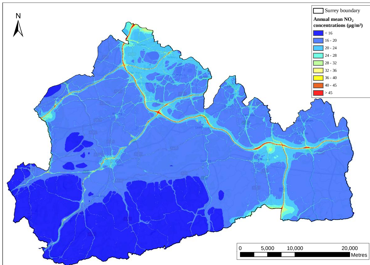
Figure 8.1: Annual mean NO 2 concentrations, 2017 (µg/m 3 )
